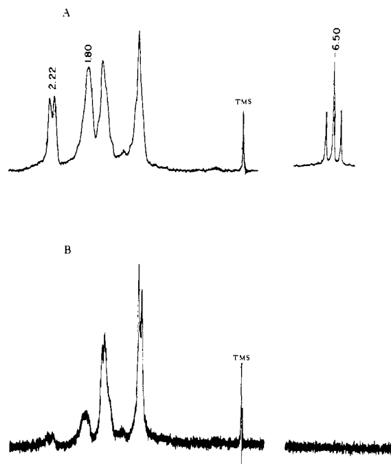
Figure 1. (A) ^1\text{H} NMR spectrum (220 MHz) of \text{ReH}_7(\text{PCy}_3)_2 in \text{C}_6\text{D}_6 . Chemical shifts ( \delta ) are noted. (B) ^1\text{H} NMR spectrum (220 MHz) of \text{ReH}_7(\text{PCy}_3)_2 after 14 h at 60 °C in \text{C}_6\text{D}_6 .
