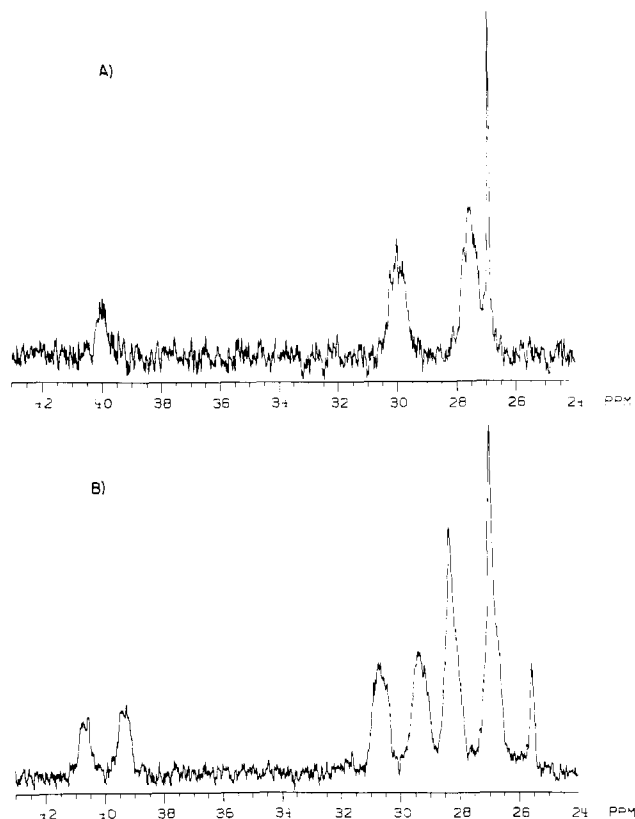
Figure 3. (A) The ^{13}\text{C}\{^1\text{H}\} spectrum of \text{ReH}_7(\text{PCy}_3)_2 after hydrogen/deuterium exchange for 1 h at 80 °C in \text{C}_6\text{D}_6 . (B) Same sample, but proton coupled.
